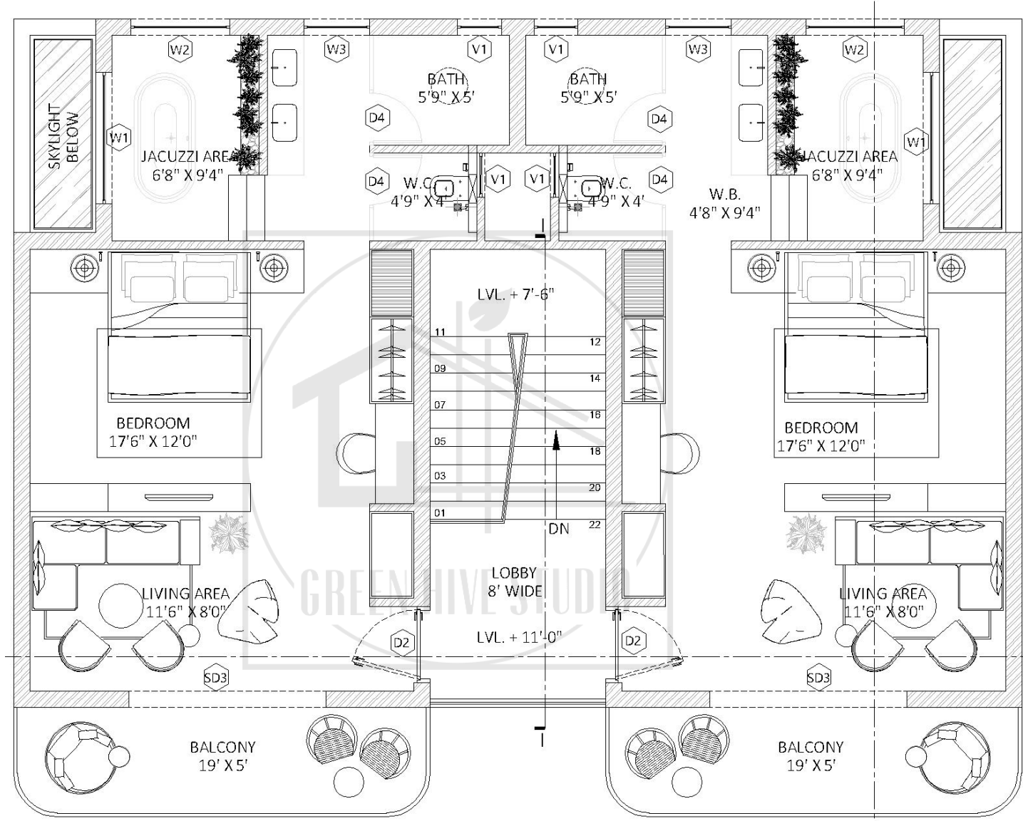
FIRST FLOOR AREA:- 645 SQFT.
