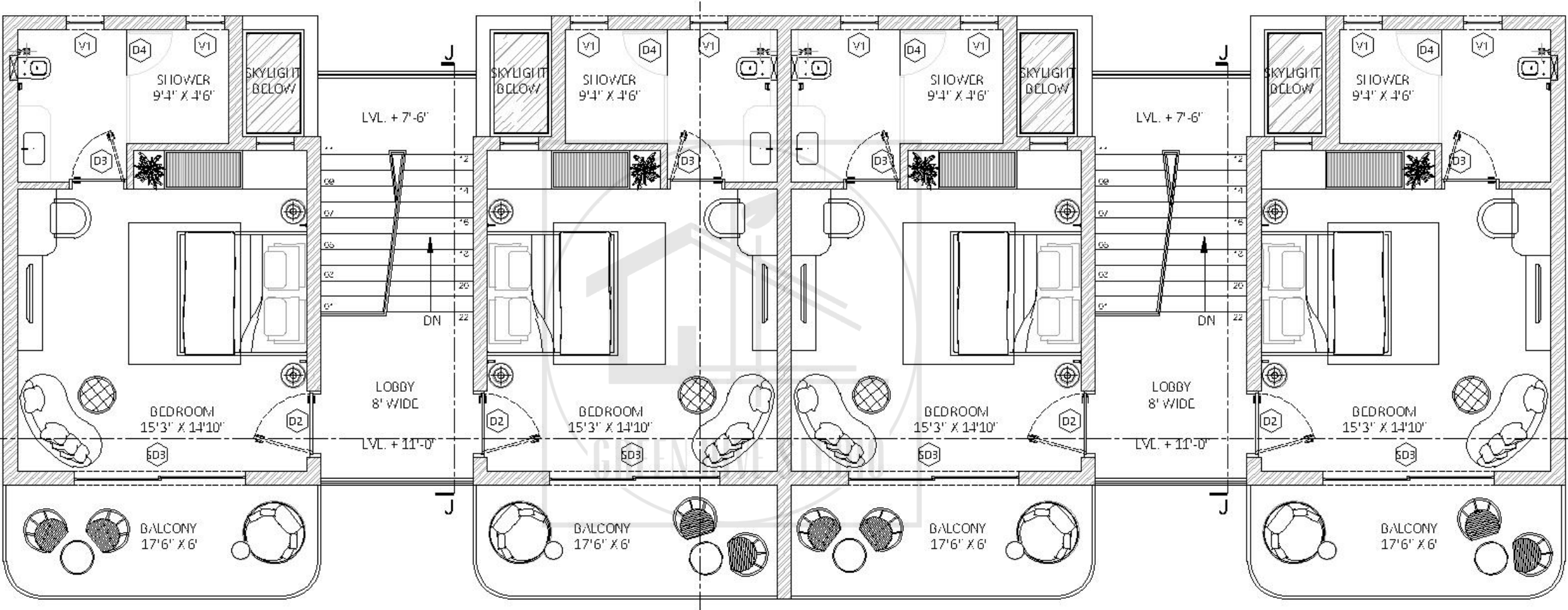
FIRST FLOOR AREA:- 450 SQFT.
